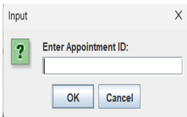
Fig 6: Cancel Appointment
