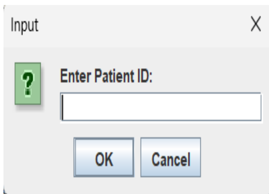
Fig 5: Search Patient
