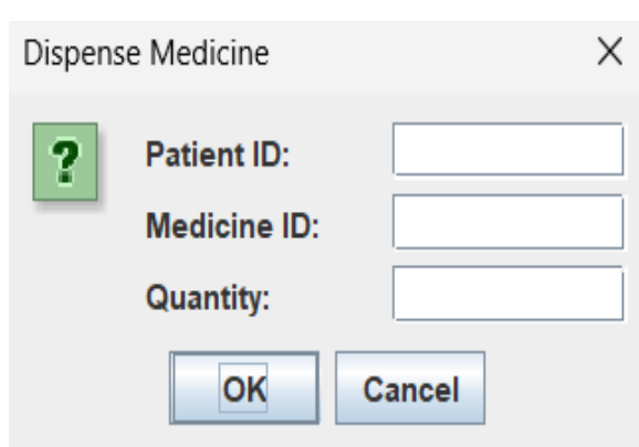
Fig 4: Dispense Medicine
