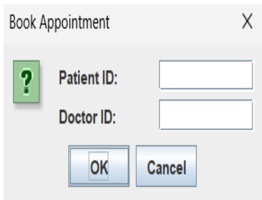
Fig 3: Book Appointment
