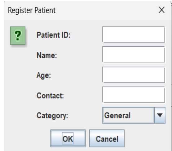
Fig 2: Register Patient
