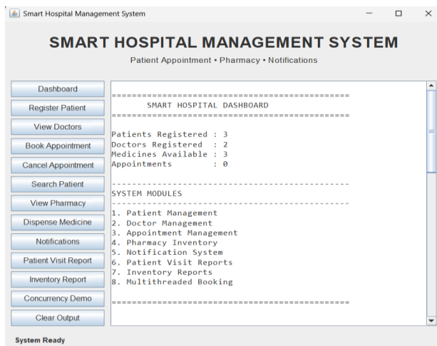
Fig 1: Dashboard
